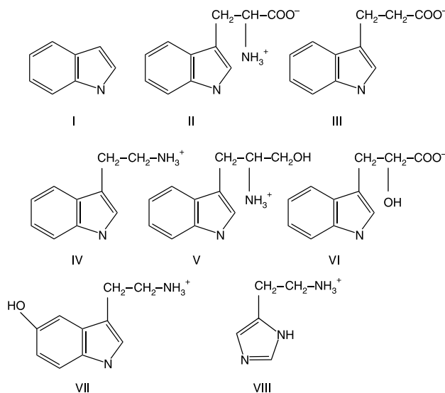
Scheme 1. Chemical structure of several indole and imidazole compounds tested for inhibition of arginase activity. I = Indole, II = L-tryptophane, III = indole-3-propionic acid, IV = tryptamine, V = tryptophol, VI = indole-3-L-lactic acid, VII = 5-hydroxy-tryptamine and VIII = histamine
