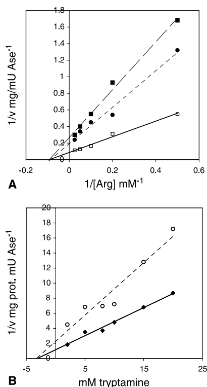
Fig. 2. Kinetic properties of the inhibitory effect of tryptamine and L-tryptophane on arginase. Tryptamine caused a noncompetitive inhibition as evidenced by double reciprocal plot (A), □ non-inhibited reaction, ■ reaction inhibited with 5 mM tryptamine, ◆ 10 mM L-tryptophane. According to the Dixon plot (B), the K_i of tryptamine is 3.1 mM. The Dixon plot supports the inhibitory mechanisms proposed by double reciprocal plots. ○, 10 mM L-arginine, ◆ 100 mM L-arginine used as substrate for arginase determination
