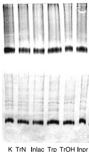
Fig. 1. Electrophoretic pattern of purified bovine and mouse macrophage arginase. Bovine arginase does not contain other detectable proteins (upper part), while mouse preparation contains mainly arginase, but a few other protein bands are also detected (below). Proteins were tested in 7% polyacrylamide gels without SDS and stained with 1% Coomassie brilliant blue G 250, dissolved in methanol/acetic acid. TrN Tryptamine, Trp L-tryptophane, Inlac indole-3-lactic acid, TrOH L-tryptophol, Inpr indole-3-propionic acid
